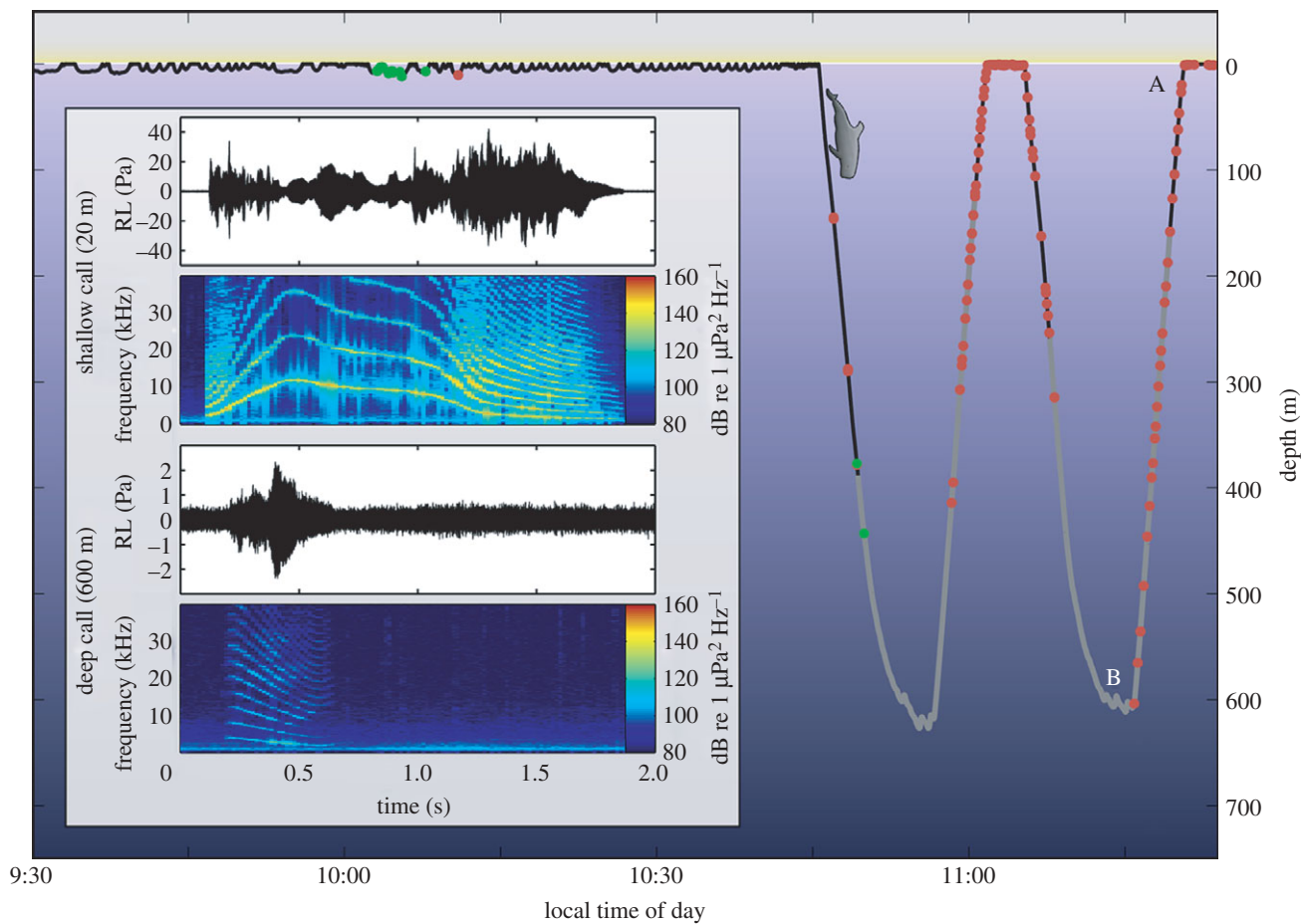
Figure 1. Annotated dive profile of a tagged short-finned pilot whale comprising a period of surface resting or socializing followed by two deep foraging dives. Two tonal calls from the last ascent (see letters in dive profile) are shown as inset waveforms and spectrograms (sampling rate 192 kHz, FFT size 4096 samples, 50% overlap): call A was produced by the tagged whale near the end of the dive, close to the surface and call B was produced at the bottom of the dive. Note the lower amplitude and shorter duration of the deep call. Grey lines, regular clicking; red dots, tonal call; green dots, pulsed call.
