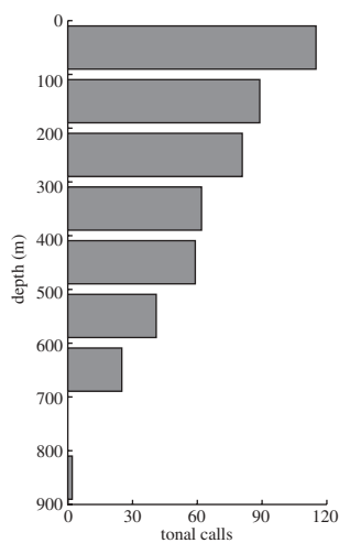
Figure 2. Histogram showing the number of tonal calls produced during deep dives by 12 tagged short-finned pilot whales ( Globicephala macrorhynchus ) as a function of depth.
