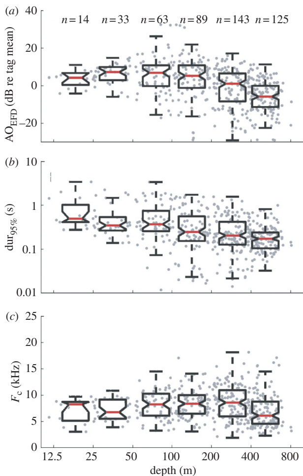
Figure 3. Acoustic parameters of tonal calls produced during deep dives by 12 tagged short-finned pilot whales ( Globicephala macrorhynchus ) as a function of depth: (a) energy flux density ( AO_{EFD} ) corrected for tag differences by subtracting mean tag values; (b) 95% energy duration ( dur_{95\%} ) and (c) centroid frequency ( F_c ). Pooled data points from all whales (grey) have been grouped into geometrically increasing depth bins (demarcated by depth-axis values) to form notched box plots, showing the 25th, 50th (median) and 75th percentile (lower, mid and upper lines in the box) of the calls within each depth bin. Whiskers mark the lowest and highest datum within 1.5 interquartile range. Notched boxes are centred on the mean depth of calls produced in each depth bin.
